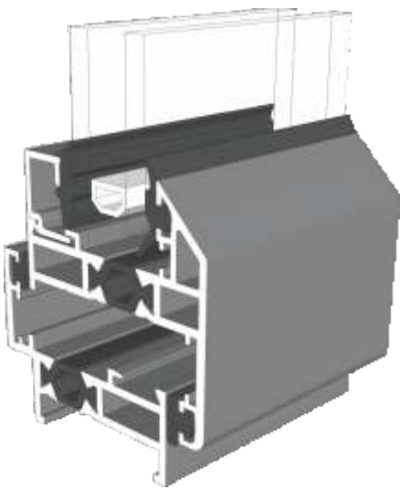
SW0052-0053 / SW0004-0030 - No Cill
