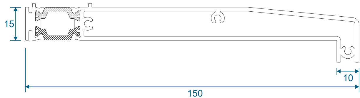
SW0022-0024 - 150mm Cill
