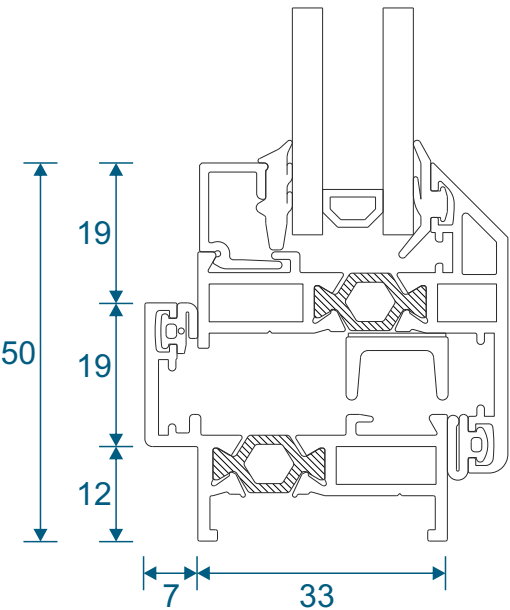
SW0052-0053 / SW0004-0030 - No Cill
