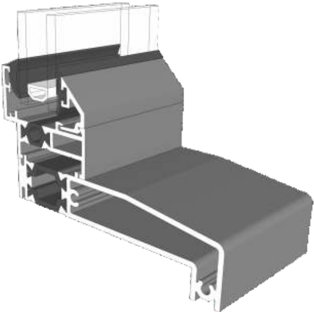
SW0052-0053 - With 85mm Cill
