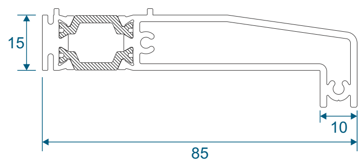
SW0022-0023 - 85mm Cill
