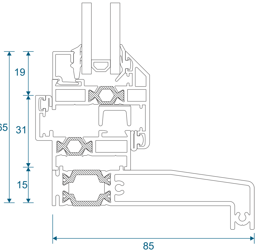
SW0052-0053 / SW0004-0030- With 85mm Cill
