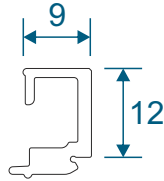
SW0012 - Handle Bead
