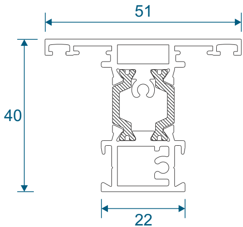
SW0050-0051 - Transom / Mullion
