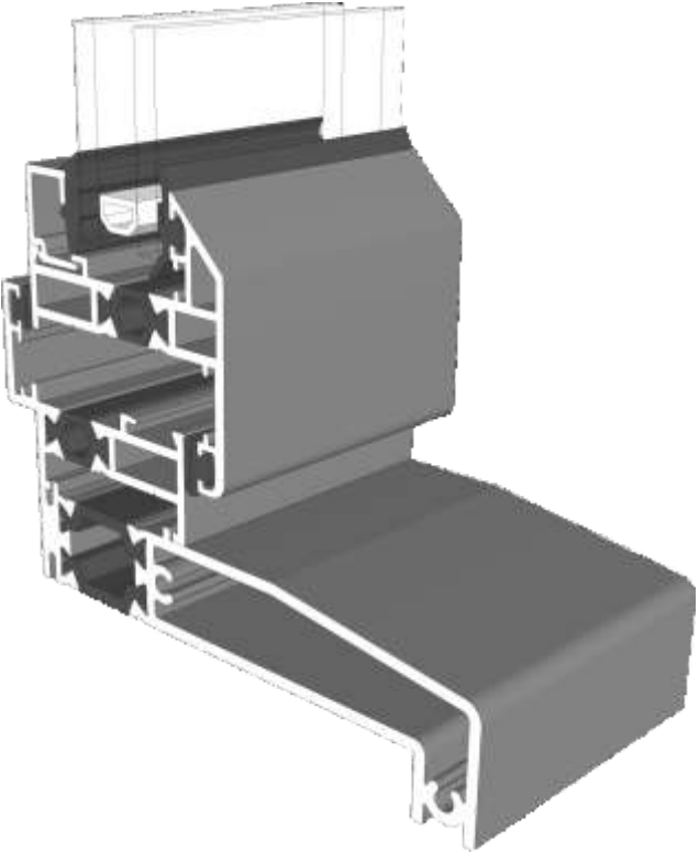
SW0052-0053 / SW0004-0030- With 85mm Cill
